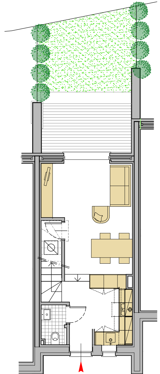
PIANO TERRA GROUND FLOOR
